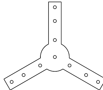
44235 12 Gauge 2-3/4" X 3/4" Legs 3/16" Holes
