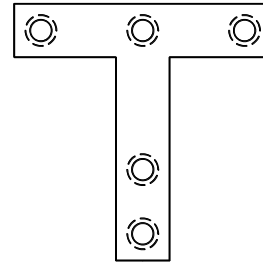
3-T 14 Gauge 3" X 3" X 5/8" \frac{1}{4} " Holes w/ CS
