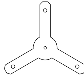
13-300 12 Gauge 3" X 3/4" Legs 1/4" Holes, 3/16" Hole
