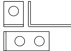
10011-B 12 Gauge 1" X 1-5/16" X 2-5/16" 1/2" Holes
