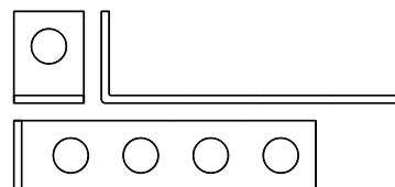
10011-D 12 Gauge 1" X 1-5/16" X 4-5/16" 1/2" Holes
