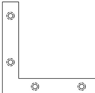
5-L 14 Gauge \frac{7}{8} " X 5" X 5" \frac{1}{4} " Holes w/ CS
