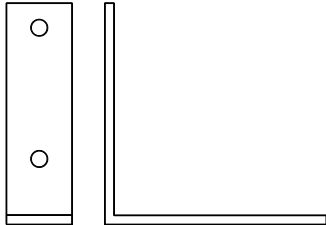
13875 12 Gauge 7/8" X 3-3/4" X 3-3/4" 3/16" Holes
