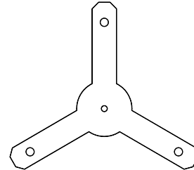
13-250 12 Gauge 2-1/2" X 3/4" Legs 1/4" Holes, 3/16" Hole
