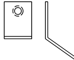
5845 16 Gauge 5/8" X 1" X 1" at 135 Degrees 3/16" Holes
